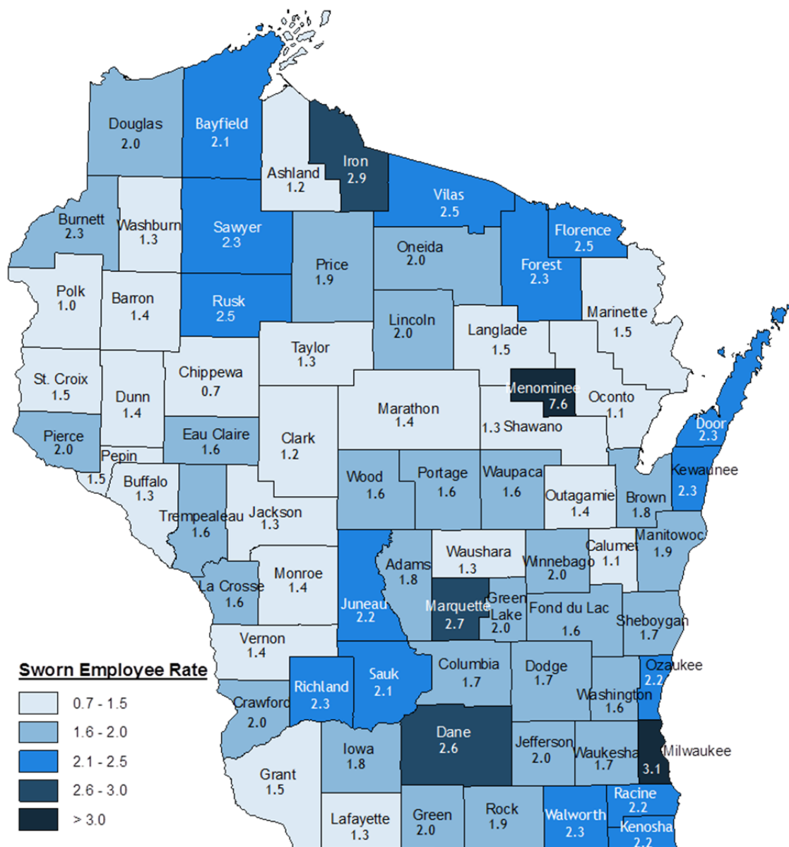
Figure 3: Rate 1 of Full-Time Sworn Employees per 1,000 Residents
